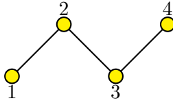
Figure 1: Example of a hierarchy with 4 players, referred to as the “N” example
