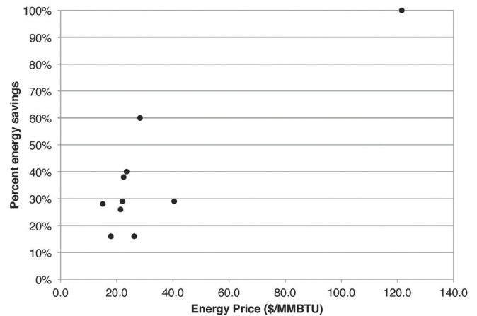
Figure 4 Percent savings over baseline versus energy price per MMBtu (MJ) for GSA NDER projects.
