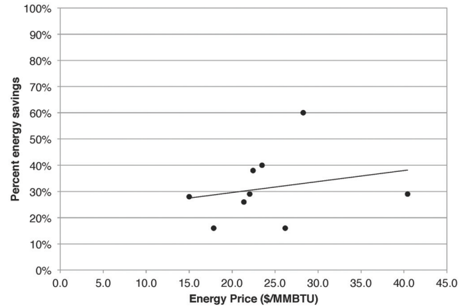
Figure 5 Percent savings over baseline versus energy price per MMBtu (MJ) for GSA NDER projects, excluding the net zero project.
