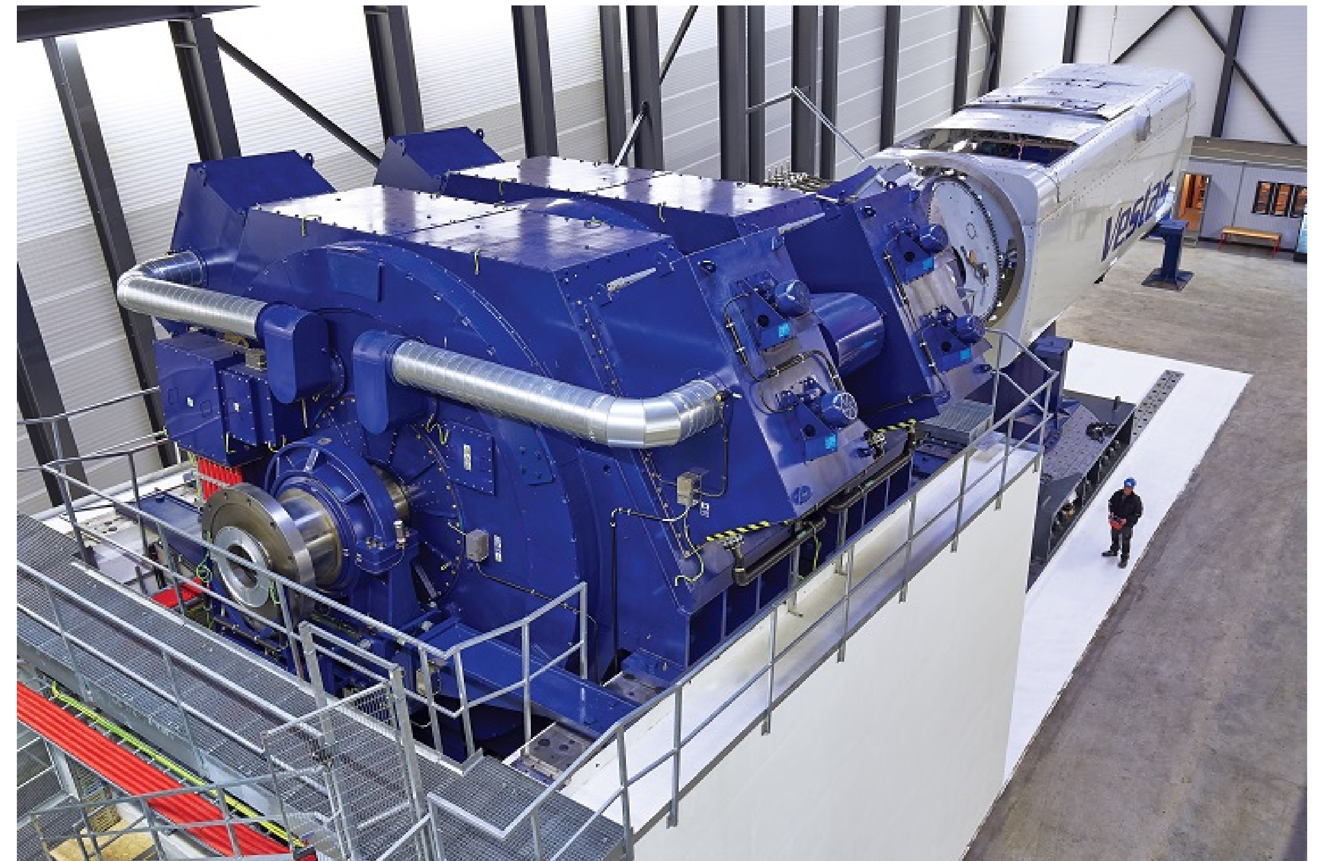
Figure 2: Function Test Bench installation at LORC, a Vestas turbine can be seen installed on the test bench.
