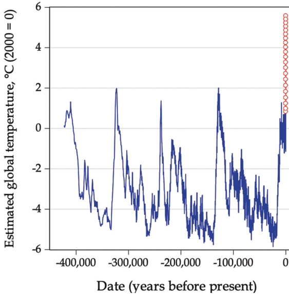
Figure 3. Estimated global temperature variations for the last 400,000 years based on Antarctic ice core (solid line) along with model projections for the next two centuries (circles). Source: Nordhaus 2013a.
