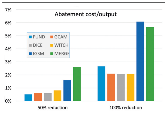
Figure 4. Abatement costs, six studies The six models as well as the methods are described in Gillingham et al. 2018. Note that the policies are harmonized across countries and assume efficient policies and 100% participation.
