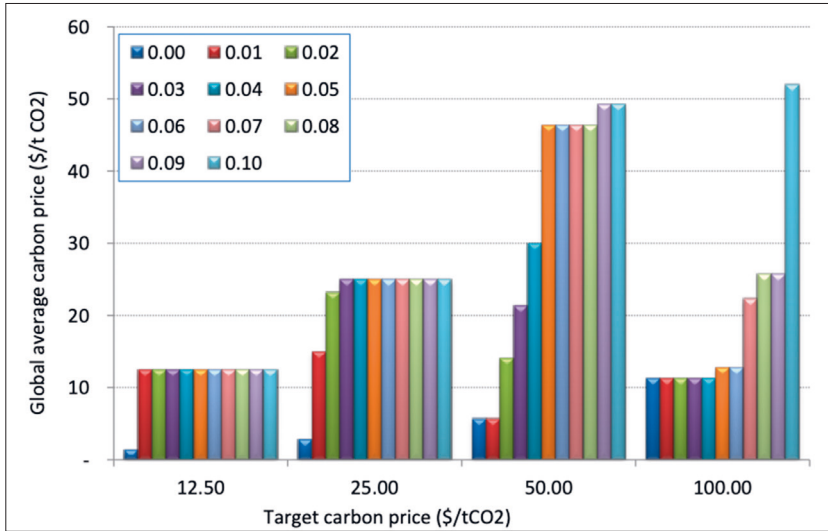
Figure 7. Actual global carbon price as a function of the target price and the penalty tariff rates
