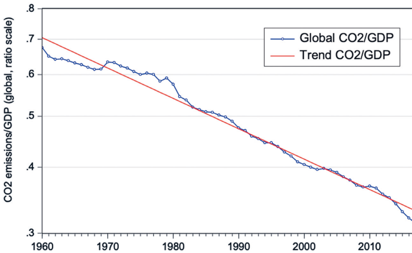
Figure 6. Trend in global decarbonization, 1980–2017.
