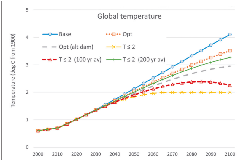
Figure 5. Temperature trajectories for different objectives.
